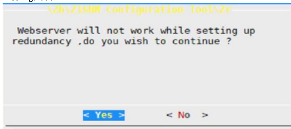
Figure 2: SNM Configuration
