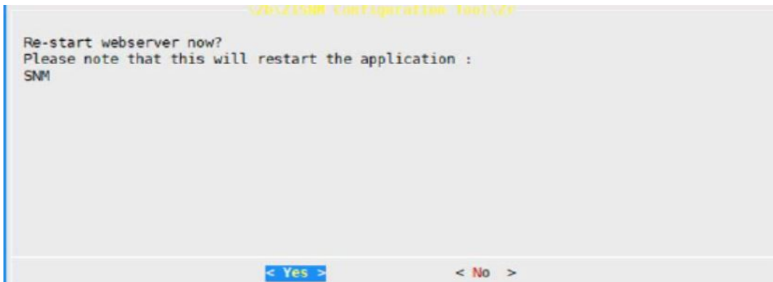
Figure 13: Webserver Restart
