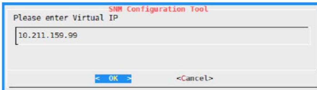
Figure 6: Virtual IP
