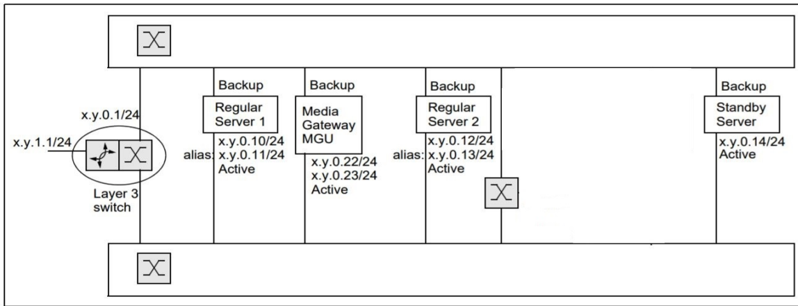
Figure 2: Server redundancy without network redundancy
