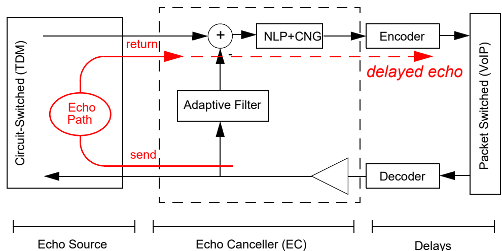
Figure 7: Schematic figure of Echo Canceller
