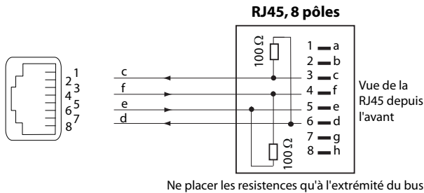
Fig. 54 Raccordement RJ45, prise simple
